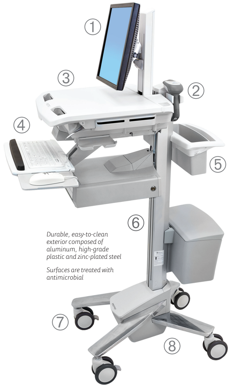
SV41 LCD Pivot cart shown with optional SV Storage Bin and optional SV Primary Storage Drawer, Single
